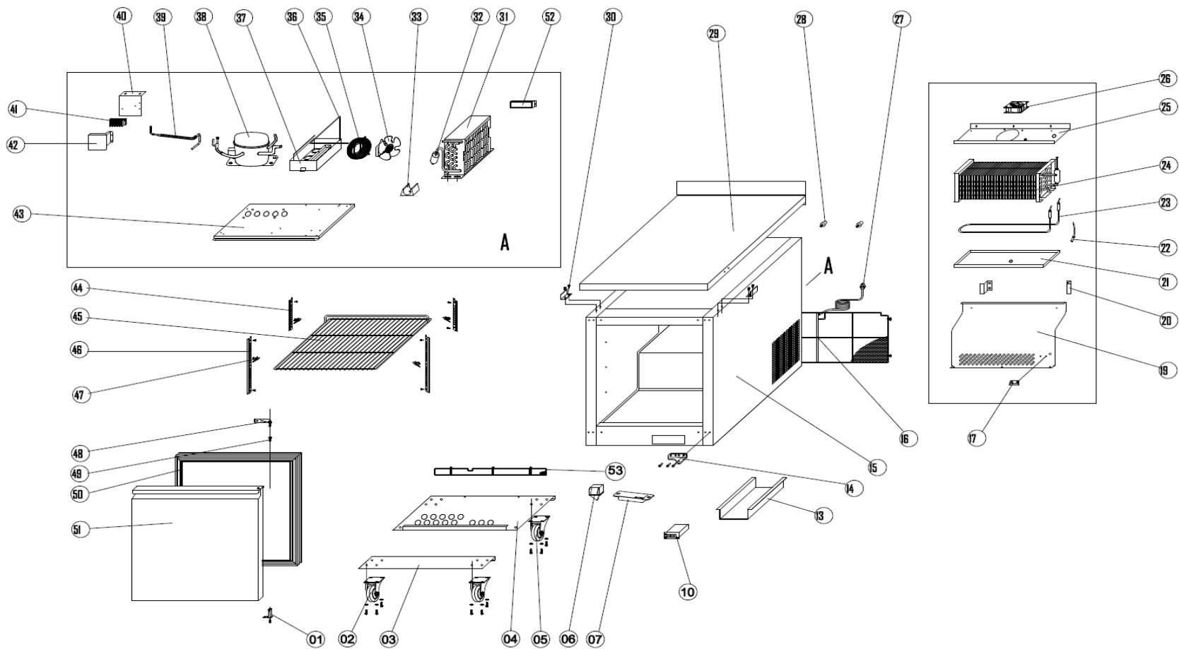
EXPLODE OF KCHUCWT27F
